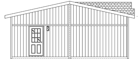
REAR ENDWALL
